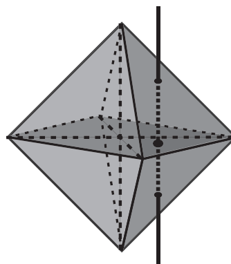
FIGURE 2. \mathcal{G}r_2^+(\mathbb{R}^7)//T^2
