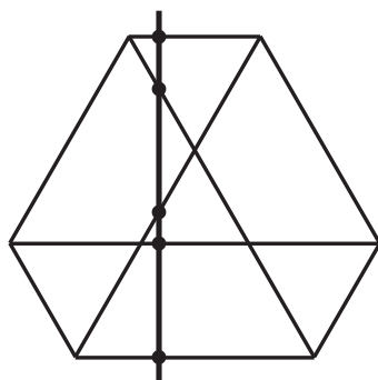
FIGURE 1. \mathcal{F}lags(\mathbb{C}^3)//S^1
