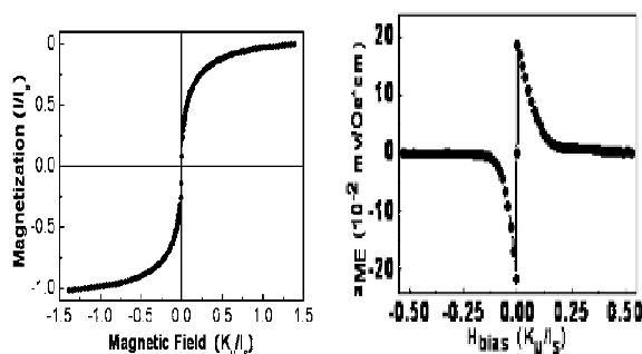
FIGURE 4. Magnetic properties of a [\text{BaTiO}_3]_{50} - [\text{CoFe}_2\text{O}_4]_{50} Bi-Crystal.
