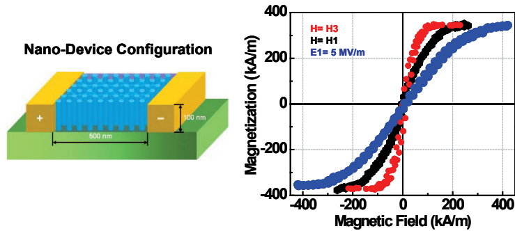
FIGURE 3. left, schematic of an electroded [\text{PS}(\text{PZT})]_{65} -block- [\text{PEO}(\text{CFO})]_{35} sample. The electric field E_1 was applied at the electrodes marked "+" and "-". Right, ferromagnetic and ME characteristics of the hexagonal CFO cylinder array embedded in the PZT matrix magnetized parallel and perpendicular to their axes, H_3 , red, and H_1 , black, and, with an applied magnetic, H_3 plus electric field, E_1 , blue. The permeability of the nanostructure can be changed by the application of an electric field. The ratio of the initial permeabilities, \mu(H_3)/\mu(H_3 + E_1) \approx 500\% .
