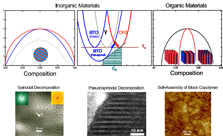
FIGURE 1. Principles of Self-Organization of Magnetolectric Nanocomposites
