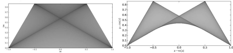
FIGURE 2. Numerical shadow for the operator
