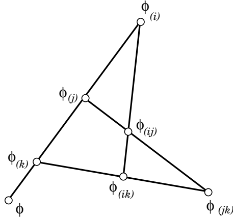
FIGURE 1. Desargues map condition and the Veblen configuration
