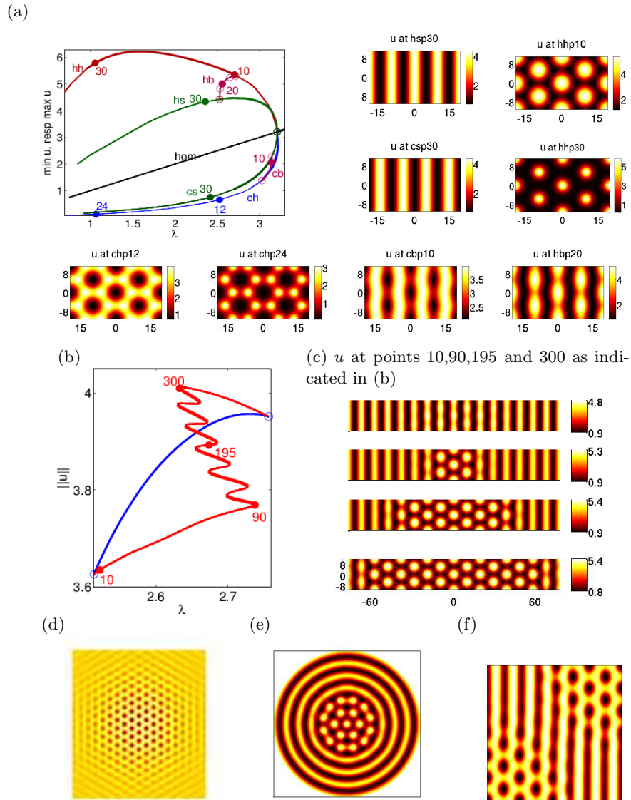
FIGURE 1. (a) “Basic” Bifurcation diagram and example solutions of (1) obtained with pde2path over the “ 2 \times 2 ”-domain. (b), (c) Bifurcation of a snaking branch of hexagons over stripes from the hb mixed mode branch (blue) over the 8 \times 2 domain, \|u\| = \|u\|_{L^8} := \left(\frac{1}{|\Omega|} \int_{\Omega} |u(x,y)|^8 d(x,y)\right)^{1/8} . (d)-(f) u for fully localized spot patterns over homogeneous background, and over radial and straight stripes. See [3] for details.
