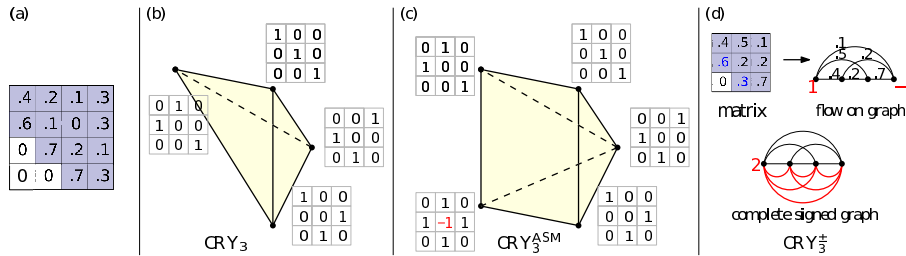
FIGURE 1. (a) A doubly-stochastic matrix in CR_{\mathcal{Y}_4} , (b) the polytope CR_{\mathcal{Y}_3} , (c) the polytope CR_{\mathcal{Y}_3}^{ASM} , (d) map from a matrix in CR_{\mathcal{Y}_3} to a flow on K_4 ; graph K_4^{\pm} associated to CR_{\mathcal{Y}_3}^{\pm} .
