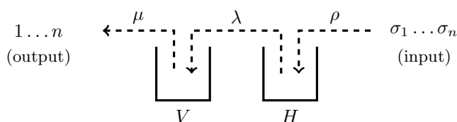
FIGURE 2. Sorting with two stacks in series.
