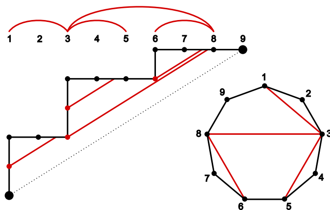
FIGURE 1. An example of a “rational triangulation”
