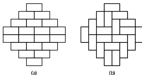
FIGURE 1. (a) The Aztec diamond of size 4, with its minimal tiling consisting only of horizontal dominos; (b) Another tiling of the same region.
