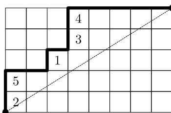
FIGURE 3. A rational parking function
