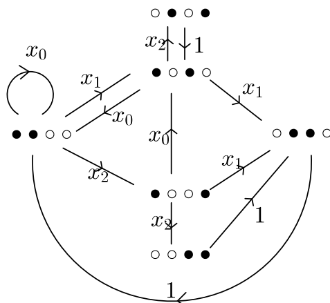
FIGURE 1. Transition graph for h = 4 and \ell = k = 2 .
