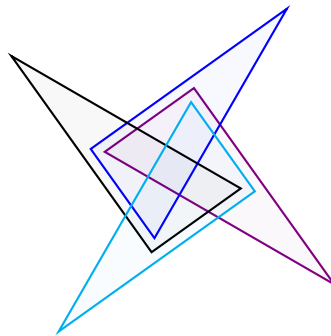
Four triangles in convex position.
