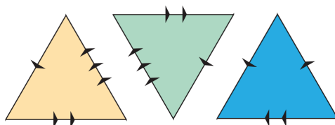
FIGURE 1. Does this 2-complex embed in \mathbb{R}^3 ?
