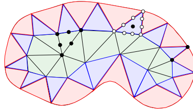
FIGURE 1. A triangulation of a curved domain with ordinary triangles (green), pie-shaped triangles (pink) and buffer triangles (blue), with the sets of domain points D_{d,T} , D_{d-1,T}^* , D_{d+1,T}^0 for d = 2 shown on one triangle of each type.
