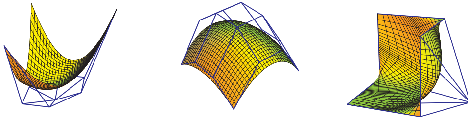
FIGURE 1. Toric Bézier patches
