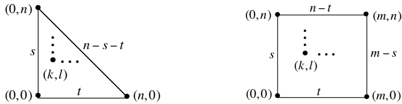
FIGURE 2. Polygons with three and four sides.
