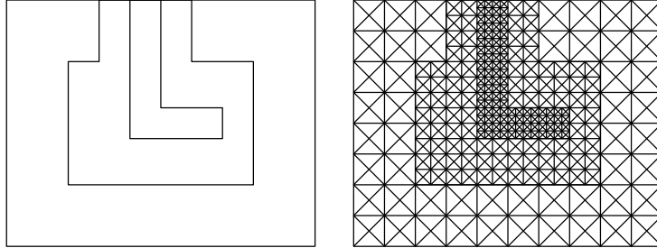
FIGURE 2. Hierarchy of nested domains (left) and the hierarchical grid defined by it (right).
