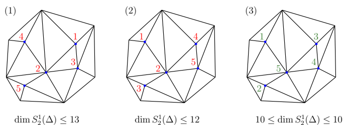
FIGURE 1. Effect of the numbering on the upper bound.
