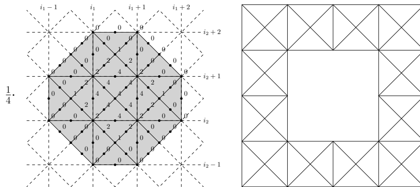
FIGURE 1. Left: Bernstein-Bézier coefficients defining a Zwart-Powell element. Right: The multicell domain from Example 1.
