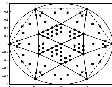
FIGURE 2. MDS for C^1 quintic macro-elements vanishing on a curved boundary. Circles, diamonds: usual MDS points for C^1 quintics on ordinary triangles. Squares: points of degree 4 on curved triangles. Triangles: points of degree 6 on buffer triangles.
