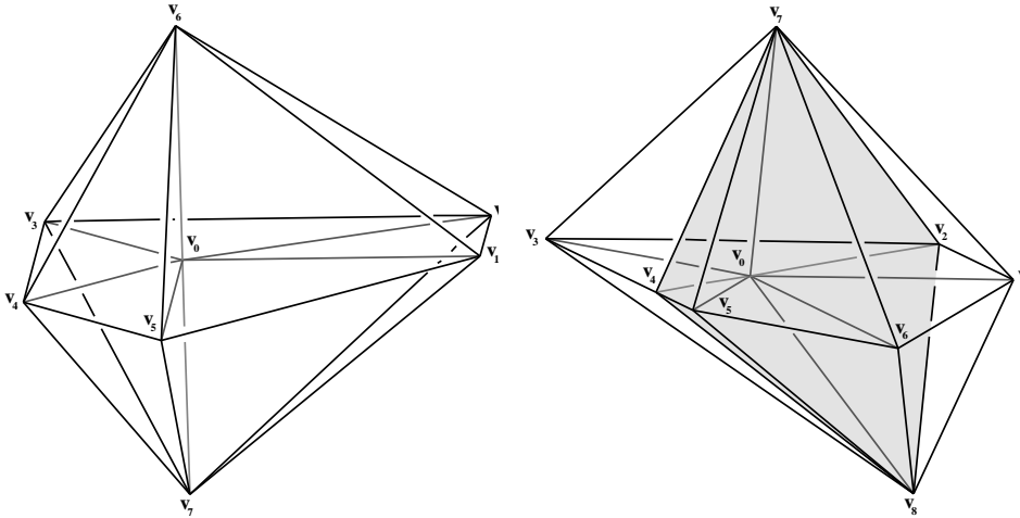
FIGURE 1. Collinear (left) and coplanar II (right) cases
