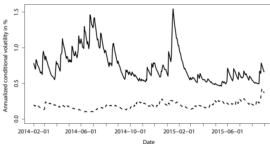
FIGURE 2. Annualized conditional volatility in % of — CRIX and - - - DAX
