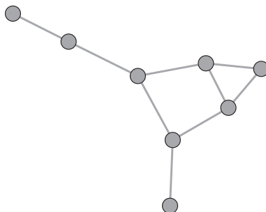
FIGURE 1. The graph \mathcal{M}(S) when g = 2 and n = 1 .
