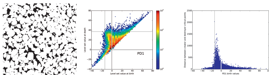
FIGURE 1. Single slice image of a sandstone. A histogram of birth and death values of the persistence diagram for dimension 1 (PD1). A scatter plot of PD1 distances between locations of the paired birth and death critical points versus their birth critical values. The pale grey vertical and horizontal lines mark percolation thresholds in the pore and grain phase respectively.
