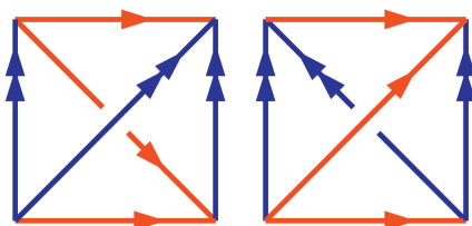
FIGURE 1. An ideal triangulation.
