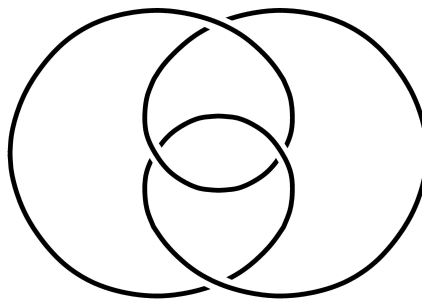
FIGURE 2. Diagram of the figure-eight knot.
