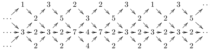
FIGURE 1. A frieze in type D_5 .
