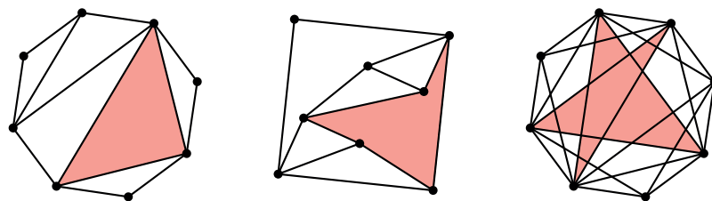
FIGURE 3. A triangle (left), a pseudotriangle (middle), and a 2-star (right).
