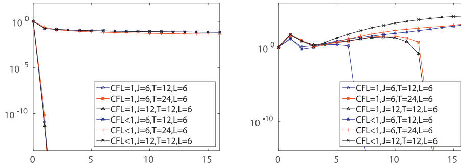
FIGURE 2. Decay of the error as a function of the number of double sweeps when using approximations of the optimal alternating Schwarz waveform relaxation algorithm
