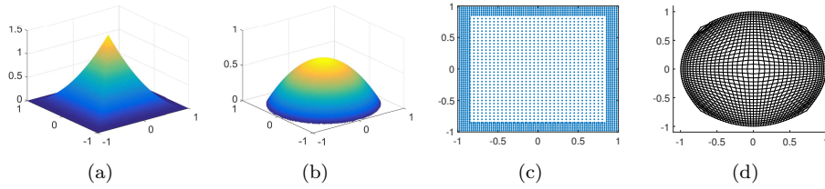
FIGURE 2. (a) Source and (b) target densities that vanish on the boundary. (c) Non-uniform mesh that resolves boundary layers and (d) computed quadratic optimal transport map.
