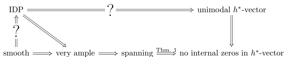
FIGURE 1. The conjectured implications are known as the Unimodality Conjecture in Ehrhart Theory and (a special case of) Oda's Conjecture . The rightmost horizontal implication in the second row follows by Theorem 1 and can be considered as a modest analogue of the unimodality conjecture.
