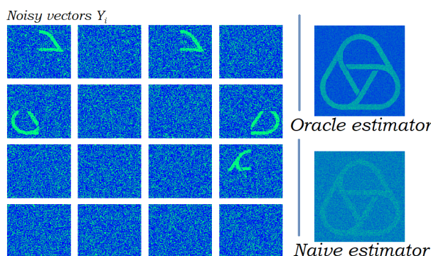
FIGURE 1. An illustration of the problem of linear functional estimation. In this example n = 10^3 , p = 5 \times 10^4 and s = 50 . We show on the left a subsample of 16 vectors Y_i each of which is obtained by vectorizing the corresponding image and, on the right, the results obtained by the naive estimator \sum_{i \in [n]} Y_i and the oracle estimator \sum_{i: \theta_i \neq 0} Y_i .
