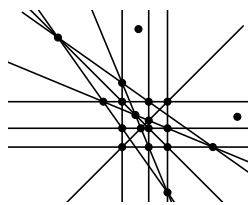
The configuration C_2
