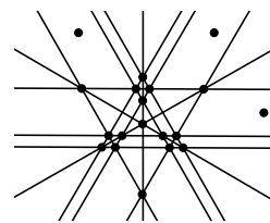
The configuration C_7
