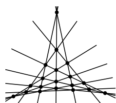
The Böröczky configuration of 12 lines
