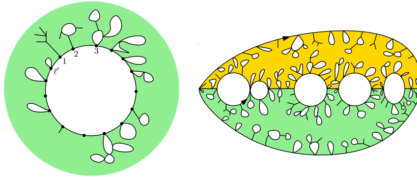
FIGURE 1. The coloured faces are the boundaries.
