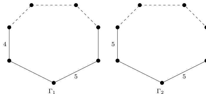
FIGURE 1. The groups \Gamma_1 and \Gamma_2 acting cocompactly on \mathbb{H}^4 . 1
