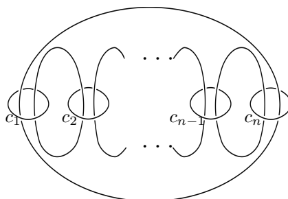
FIGURE 1. \mathrm{FAPL}_n , with crossing circles c_i , i = 1, \dots, n .
