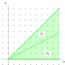
FIGURE 1. The chamber complex of a piecewise quasipolynomial.
