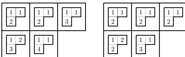
FIGURE 1. Examples of plethystic tableaux
