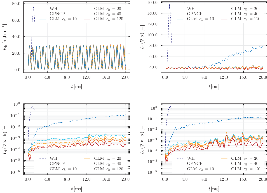
FIGURE 1. Time evolution of global dynamics and of curl errors for an oscillating bubble. Top row, left to right: total kinetic energy and L_1 norm of the gradient field \nabla \mathbf{b} over time. Bottom row: the timeseries for the L_1 and L_2 norms of the curl error. The simulations employed a sixth order ADER-DG scheme with third order ADER-WENO subcell finite volume limiter uniform Cartesian grid composed of 64^2 elements.
