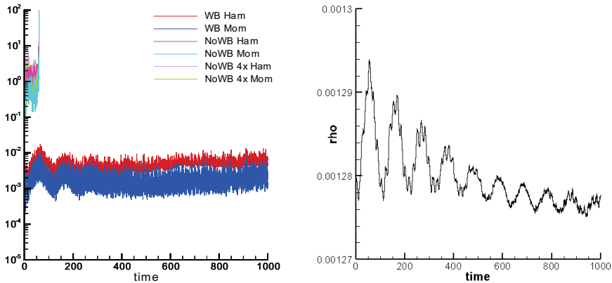
FIGURE 1. TOV star simulation with the CCZ4+GRHD fully coupled model corresponding to an initial perturbation over the pressure profile p . Left: we show the values of the Hamiltonian and momentum constraints which are close to machine precision and constantly maintained for long computational times with the WB code, while they rapidly blow up with the not WB code. Right: we plot the numerical results obtained with the new WB scheme for the density of the star at an inner point with r = 0.5 which oscillates due to the initial pressure perturbations.
