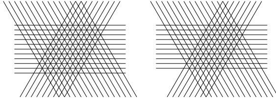
FIGURE 4. The arrangements \mathcal{A}_{\text{Cat}}^{\mathbf{k}} and \mathcal{A}_{\text{Shi}}^{\mathbf{k}} for \mathbf{k} = (1, 3, 4) .
