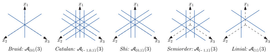
FIGURE 1. The braid, Catalan, Shi, semiorder, and Linal arrangements in dimension n = 3 (seen from the direction (1, 1, 1) ).
