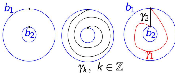
FIGURE 1. An annulus with two marked points and its curves
