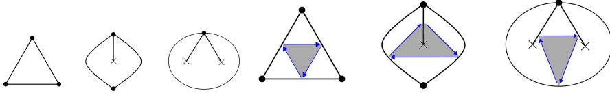
FIGURE 1. Left: The tree types of triangles of a triangulation. Right: The cells of the CW-complex X(\tau) = (X_n(\tau))_{n=0,1,2} .
