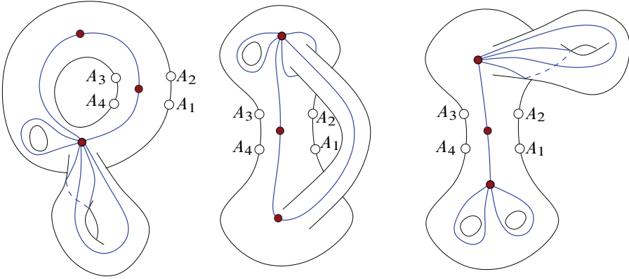
Figure 2.3. Embedding a graph G in the Seifert surface. In each case, the Seifert surface deformation retracts to a neighborhood of G that contains A_1 A_2 A_3 A_4 .
