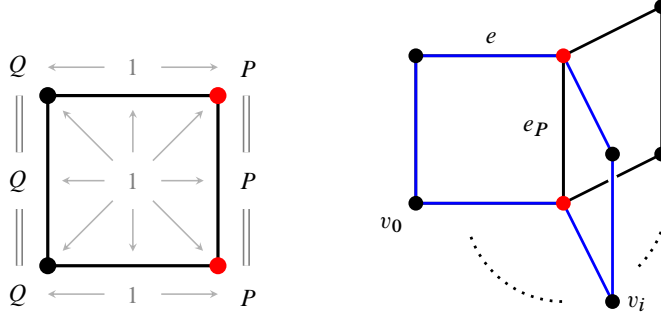
Figure 1. The complex of \mathcal{G}(P, Q) is the complex of groups with indicated local groups and a portion of the development around the edge stabilized by P . The blue circuits pass through e and v_i for i \geq 1 , but all have peripheral backtracking because they are separated by the subcomplex \Sigma_P = e_P with red endpoints.
