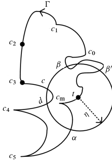
Figure 1. Diagram of \Gamma_\eta = \widehat{\alpha\beta} + \widehat{c\delta} .
