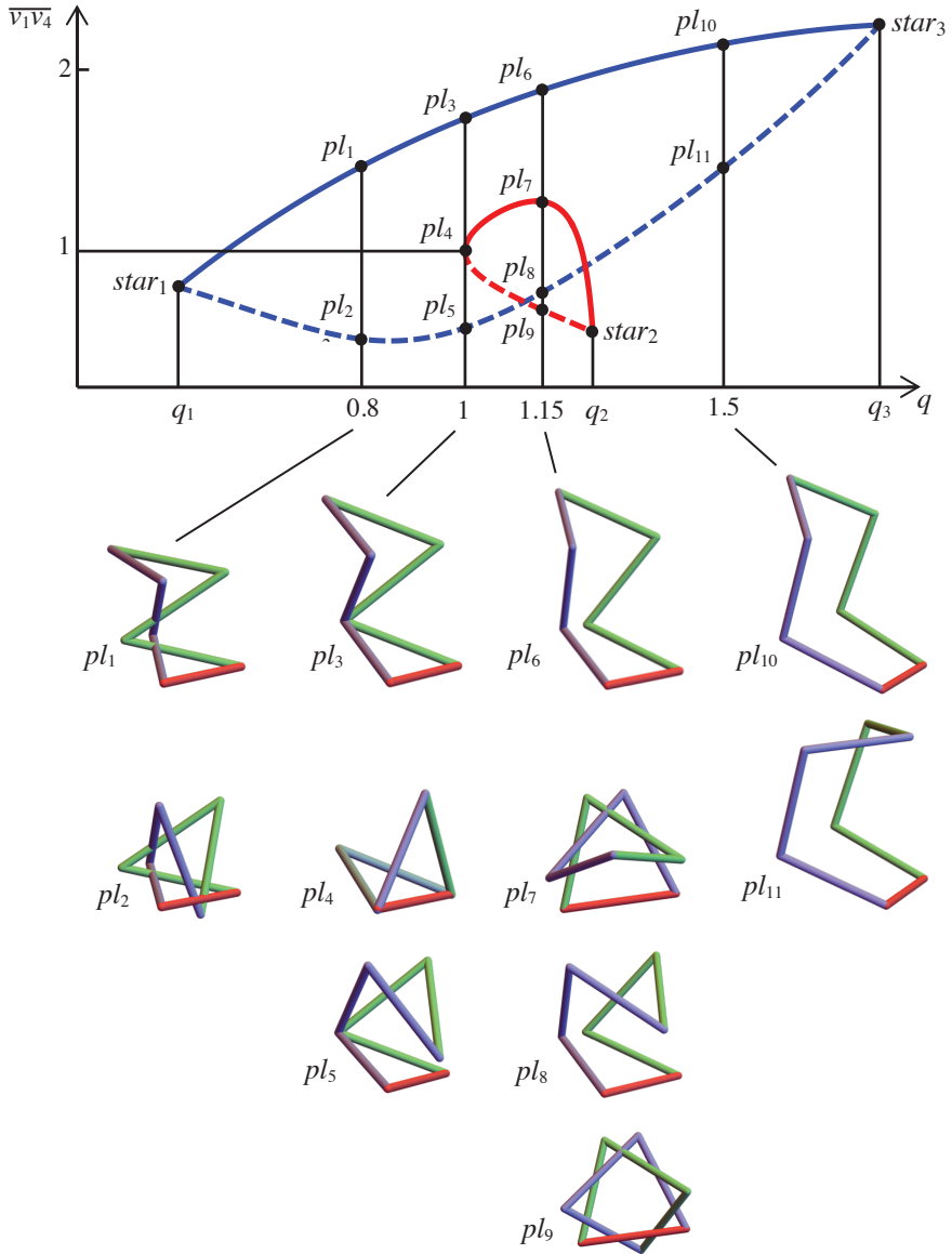
Figure 3. Plane-symmetric heptagons represented by diagonal pairs (q, \sqrt{v_1 v_4}) , with examples of some selected values of q .
