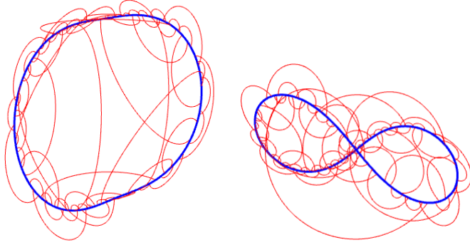
Figure 9. Two views of an approximation of the crown \text{Crown}_{\Gamma, \gamma} , where \Gamma is the \mathbb{R} -Fuchsian (3, 3, 4) -triangle group, and \gamma is the word \iota_3 \iota_2 \iota_1 \iota_2 (see Example 5.6). Here, the (thick) blue curve is the \mathbb{R} -circle which is the limit set of the group \Gamma . The red (thin) curves form the orbit of the axis at infinity of \gamma .
