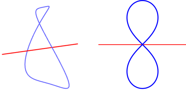
Figure 2. Two \mathbb{R} -circles: the red line is the x axis of the Heisenberg coordinates. It is the boundary of \mathbf{H}_{\mathbb{R}}^2 = \mathbb{R}^2 \cap \mathbf{H}_{\mathbb{C}}^2 . The blue curve is the boundary of a real plane orthogonal to \mathbf{H}_{\mathbb{R}}^2 . The left picture is a view in perspective in Heisenberg space, and the right picture is the vertical projection of the two \mathbb{R} -circles on \mathbb{C} .
