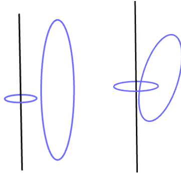
Figure 3. Examples of \mathbb{C} -circles in Heisenberg space. On both pictures, the black line is a \mathbb{C} -circle passing through \infty . Note that the pair of blue \mathbb{C} -circles on the left is unlinked, whereas in the right picture they are linked.
