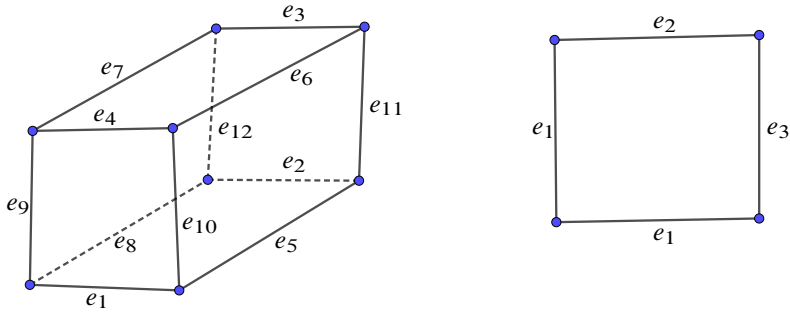
FIGURE 2 A quadrangulation of a sphere and a quadrangulation of a disc.
