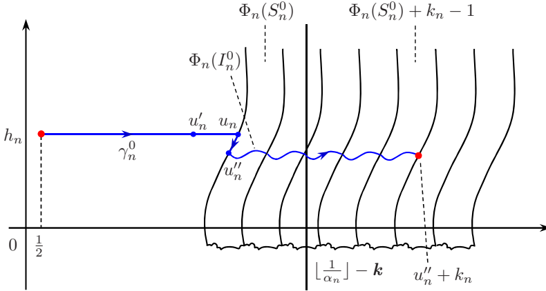
Fig. 6. The sketch of the construction of the continuous curve \gamma_n^0 (in blue) in the Fatou coordinate plane of f_n . The two red dots denote the initial and terminal points of \gamma_n^0 and they have the same image under the map \Phi_n^{-1} . In particular, \Phi_n^{-1}(\gamma_n^0) is a continuous closed curve in the Siegel disk of f_n .
