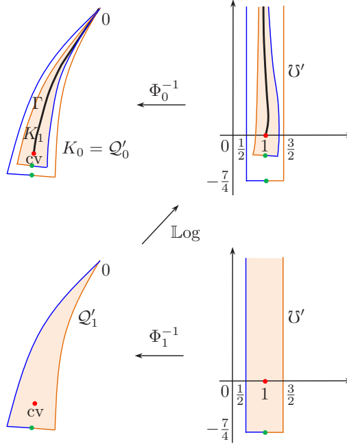
Fig. 7. A sketch of the renormalization microscope between levels 0 and 1. The sets \Gamma , U' , Q'_n , K_n with n = 0, 1 and some special points are marked.
