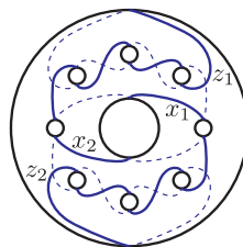
Fig. 25. The bounding quadruple.
