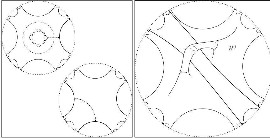
Figure 4. Representation of the surface H^0 . On the left, the leaves of type 0 and 1 used in its construction. Bold lines are the identified boundary components.
