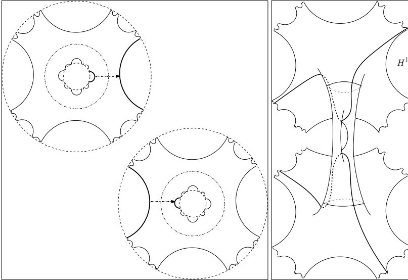
Figure 5. The surface H^1 . Outer (respectively, inner) boundary components of H^1 are the union of outer (respectively, inner) boundary components of the former two leaves of type 1. Bold lines represent the identified boundary components.
