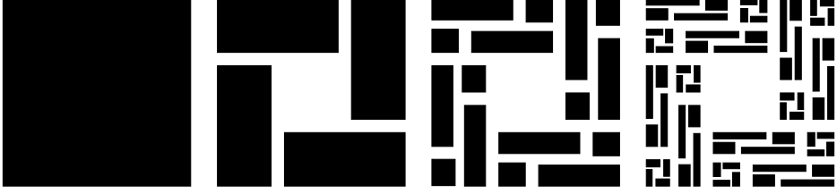
Figure 1. Mendivil–Taylor fractal
