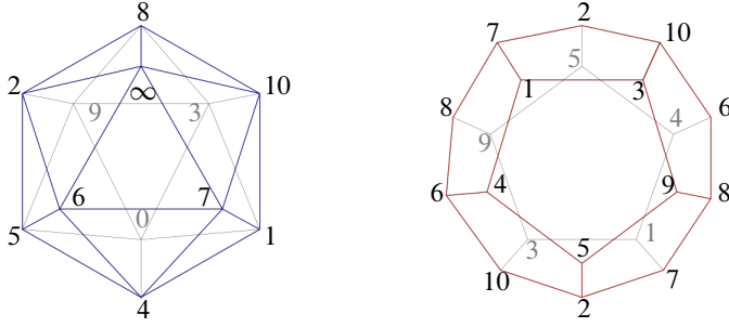
FIGURE 4 Le cas p = 11 .
