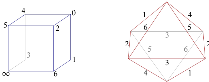
FIGURE 3 Le cas p = 7 .
