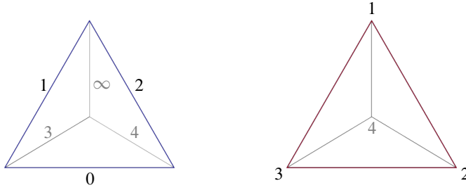
FIGURE 2 Le cas p = 5 .
