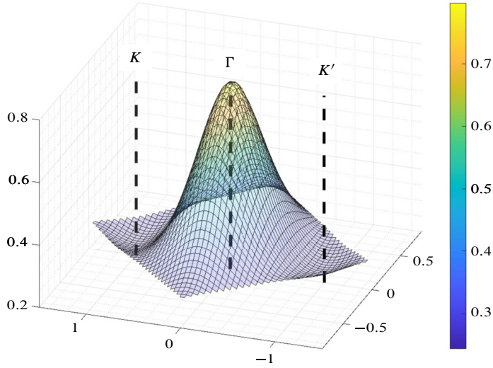
Figure 7. Open Problem 16.
