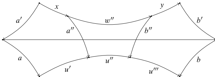
Figure 5.2. The evaluation of B\langle a, b \rangle \langle a', b' \rangle agrees with the evaluation of x \cdot B[i : j] \langle a'', b'' \rangle \cdot y . Here we are assuming that \text{eval}(B) = u = u'u''u''' and that \text{eval}(B[i : j] \langle a'', b'' \rangle) = w'' .
