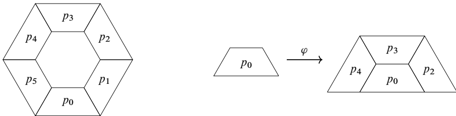
Figure 7. The half-hex prototiles are on the left and the substitution of p_0 is on the right. All other substitutions are rotations of p_0 by n\pi/3 .
