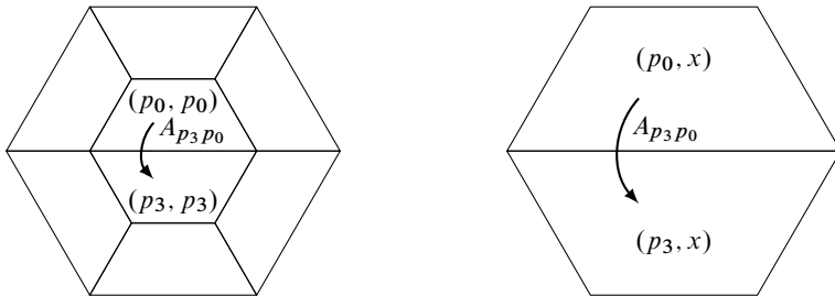
Figure 10. An illustration of the first formula A_{p_3 p_0} \cdot (p_0, p_0)w = (p_3, p_3) A_{p_3 p_0} \cdot w in (5.3) with i = 0 . The left-hand side shows the action A_{p_3 p_0} \cdot (p_0, p_0) = (p_3, p_3) and the right-hand side shows that the element A_{p_3 p_0} comes from the relationship between one-supertiles.
