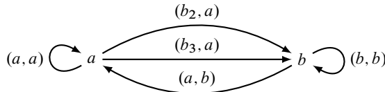
Figure 3. The supertile extension graph of Example 2.4.
