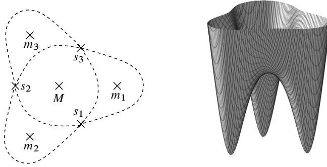
Figure 1. The structure of the critical points of f and an example of such a Morse function.
