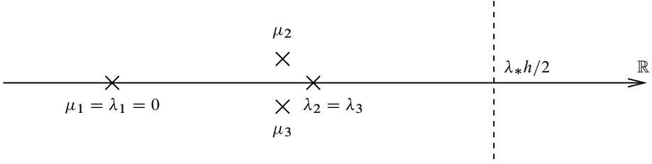
Figure 2. The low-lying eigenvalues of P_0 and P_{\text{com}} .
