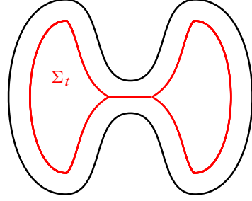
Figure 1.2. A schematic illustration of the connected curve \Sigma_t in the case of a dumbbell-like domain. The proof of Theorem 1.2 will show that the segment connecting the two connected components of S_t is doubly covered.
