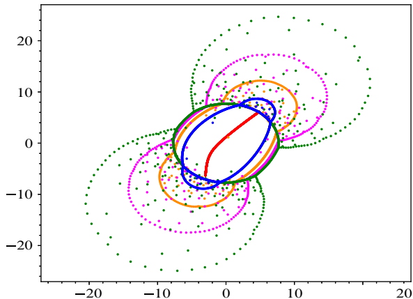
Figure 1. The set \text{sp} T_n(a) for a(z) = z^2 + cz + cz^{-1} with c = 2 + 3i and n = 1024 , computed with d precision digits for different values of d . The green, magenta, orange, blue, and red points correspond to d = 16, 32, 64, 128, and 500 , respectively.
