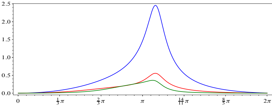
Figure 10. The absolute value of the individual normal error \text{NE}_{j,n}^{\text{SL}(k)} for n = 2048 and different values of k : k = 1 (blue), k = 2 (red), and k = 3 (green). For the eigenvalue \lambda_{j,n} = \psi(s_{j,n}) we took as independent variable s_{j,n} and plotted the errors over the grid j\pi/(n+1) for j \in \{1, \dots, n\} .
