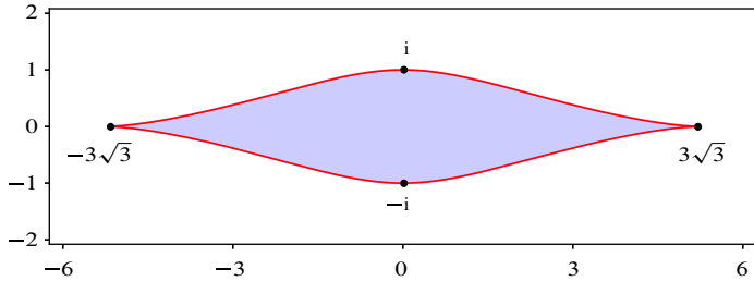
Figure 4. The set \Omega .
