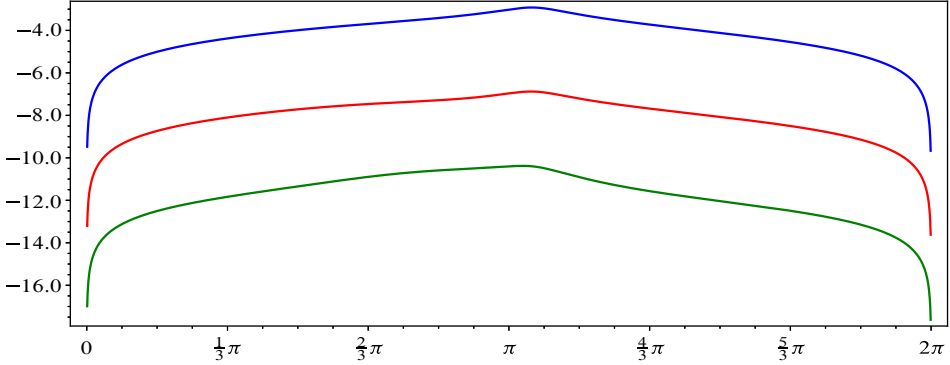
Figure 9. The 10-base logarithm of the individual relative error \text{RE}_{j,n}^{\text{SL}(k)} for n = 2048 and different values of k : k = 1 (blue), k = 2 (red), and k = 3 (green). For the eigenvalue \lambda_{j,n} = \psi(s_{j,n}) we took as independent variable s_{j,n} and plotted the errors over the grid j\pi/(n+1) for j \in \{1, \dots, n\} .
