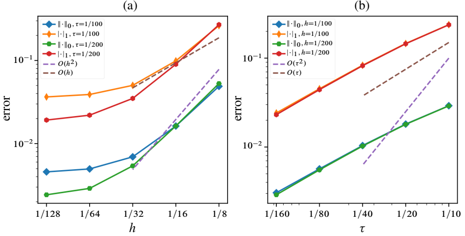
Figure 2. Errors of the phase field \varphi : (a) the x-axis corresponds to the mesh size h ; (b) the x-axis corresponds to the time step size \tau .
