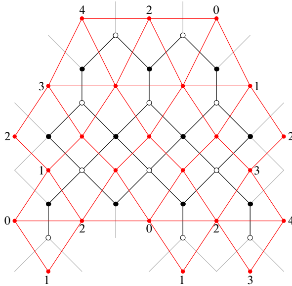
Figure 3. Contracting square-hexagon lattice \mathcal{R}(\Omega, \check{c}) , dual graph \mathcal{R}^*(\Omega, \check{c}) and height function on the boundary. The black lines represent the graph \mathcal{R}(\Omega, \check{c}) , the gray lines represent boundary edges of \mathcal{R}(\Omega, \check{c}) , the red lines represent the dual graph \mathcal{R}^*(\Omega, \check{c}) , and the height function is defined on vertices of the dual graph. The values of the height function on the boundary vertices of \mathcal{R}^*(\Omega, \check{c}) are also shown in the figure.
