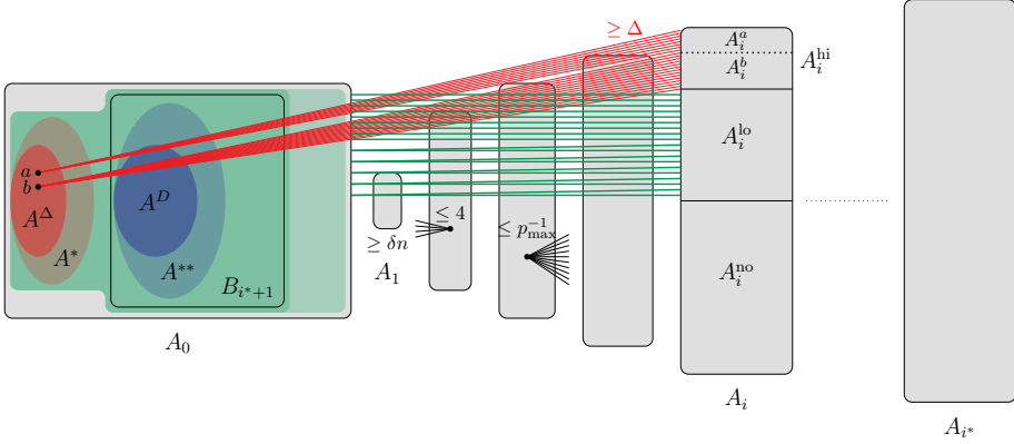
Fig. 3. Partition of F obtained in TREE PARTITION. Red edges are from T \setminus F and green edges are F -edges from A_0 to A_i (so A_i^{lo} ).
