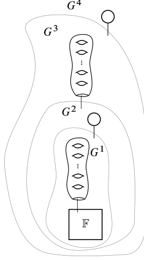
Figure 3. A tower of height 4.
