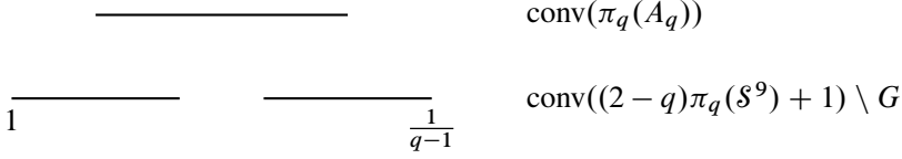
Figure 9. \pi_q(A_q) and (2-q)\pi_q(\mathcal{S}^9) + 1 are interleaved. Here, G denotes the largest gap of ((2-q)\pi_q(\mathcal{S}^9) + 1) .
