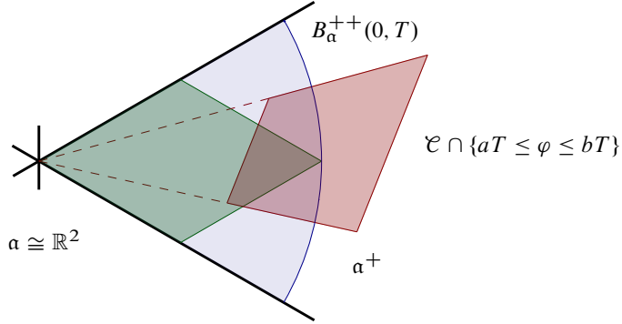
Figure 1. This is a positive Weyl chamber for \mathrm{SL}(3, \mathbb{R}) and T > 0 is large. In blue, our counting region B_{\alpha}^{++}(0, T) . In green, Deitmar–Gon–Spilioti’s [13] counting region. In red, Guedes Bonthonneau–Guillarmou–Weich’s [25] counting region where \mathcal{C} is a convex cone strictly inside \alpha^{++} delimited by the red dashed lines, 0 < a < b are real numbers and \varphi is a linear form strictly positive on \alpha^+ .
