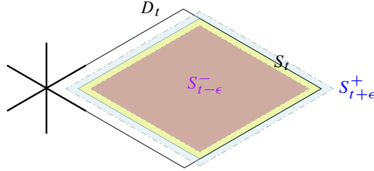
Figure 3. Parallelootope domain, S_{t+\epsilon}^+ is the blue outer layer delimited by the gray dash dots, S_t in green-yellow is the mid-layer delimited by the gray line and a portion of the black line, S_{t-\epsilon}^- is the innermost layer delimited by the gray dotted line.
