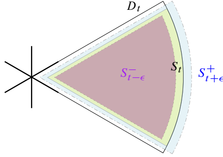
Figure 2. Ball domain, S_{t+\epsilon}^+ is the blue outer layer delimited by the dash dots, S_t in green yellow is the mid layer delimited by the gray line, S_{t-\epsilon}^- is the innermost layer delimited by the gray dotted line.
