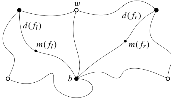
Figure 7. The definition of the height function in terms of winding.
