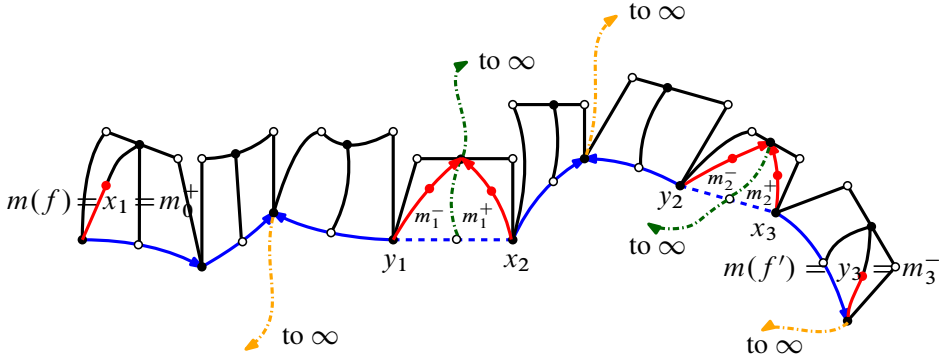
Figure 9. An example for the computation of the height along an arbitrary trajectory. The path P in \Gamma is the union of solid blue and dashed blue edges, and here, it is composed of k = 3 partitions. The solid blue denotes the segments in the tree \mathcal{T} with arrows giving the orientation of each edge. The union of solid red and solid blue edges is the modified path. The orange dotted paths denote the direction in which the primal tree goes off to \infty and the green dotted path denotes the same for the dual tree. This determines the \varepsilon'_i 's and \delta'_i 's. Here, \varepsilon_1 = -1 , \varepsilon_2 = 1 , \varepsilon_3 = -1 , and \delta_1 = 1 , \delta_2 = -1 .
