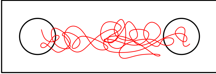
Figure 3. An illustration of the crossing condition.
