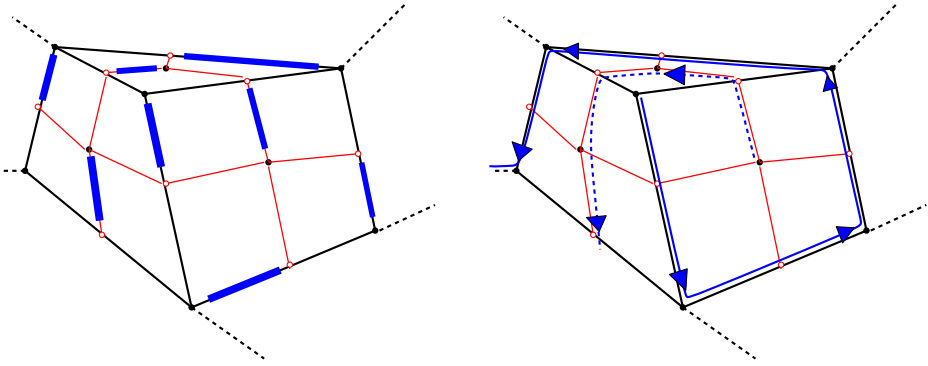
Figure 6. Illustration of the local transformation in Temperley’s bijection. Left: a dimer configuration on a superposition graph. Right: a collection of oriented edges forming dual oriented CRSF.
