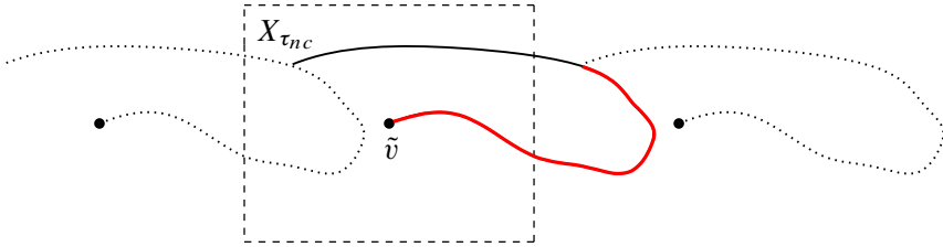
Figure 13. A schematic representation (in solid line) of the lift of the loop erasure of the random walk on the torus until a non-contractible loop is formed. Call this path \tilde{\gamma} , and let \gamma = p(\tilde{\gamma}) . The dashed square denotes the fundamental domain and the dashed paths denote some other lifts of \gamma . In this case, \tilde{\gamma} stops inside the fundamental domain.
