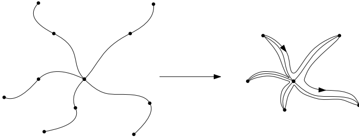
Figure 8. Proof of Lemma 4.3.
