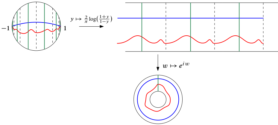
Figure 11. The conformal maps between an annulus and its universal cover. The dotted lines separate different copies of the fundamental domain. The blue and red curves show two loops in the surface and the associated spines in the cover.
