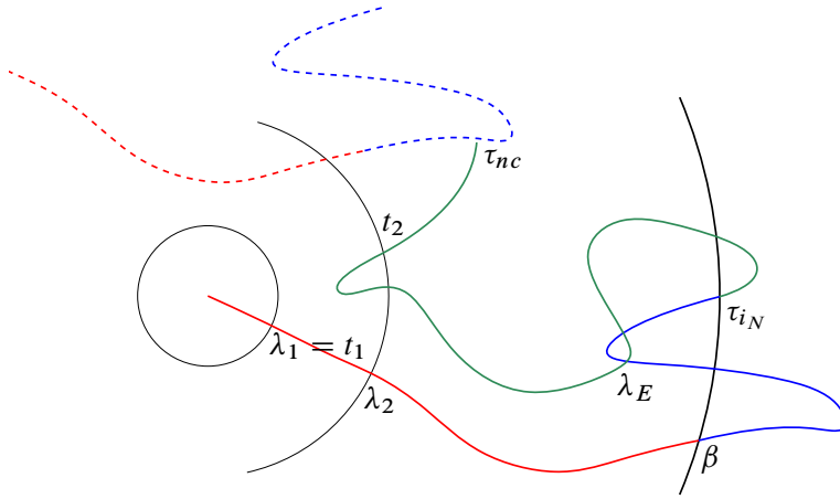
Figure 14. The concatenation of the red and blue curves is \tilde{Y}^{\tau_{i_N}} and the green part is \tilde{X}[\tau_{i_N}, \tau_{nc}] . The dotted path denotes a copy of \tilde{Y}^{\tau_{i_N}} so overall the event represented is one where a non-contractible loop is formed inside B(\tilde{v}, e^{-t_0}) .
