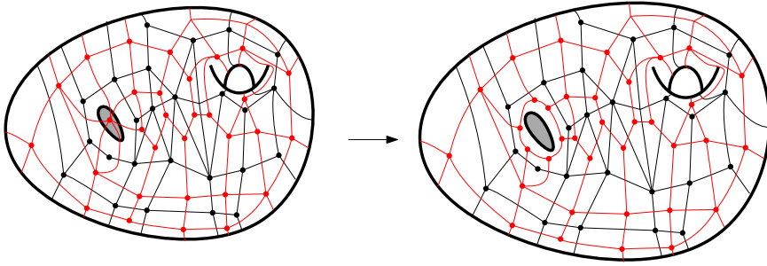
Figure 10. Splitting of the boundary vertex of \Gamma (red graph) into a cycle. The black graph is \Gamma^\dagger .
