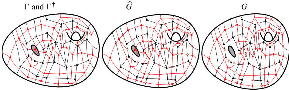
Figure 1. The graphs \Gamma , \Gamma^\dagger , \hat{G} , and G . The graph \Gamma is pictured in red and \Gamma^\dagger in black.
