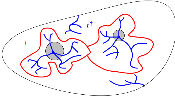
Figure 5. A non-Temperleyan CRSF (in blue). The surface M is the “pair of pants”: a domain of the plane with two holes (in grey in the picture). In this example, t does not contain any cycle, and hence, any connected component flows to the boundary of M . Its dual t^\dagger must contain a component with two cycles which overlap. The cycles go around each of the two holes and must be connected, as otherwise there would have to be a path in t separating them; however, this is impossible as such a path would have to connect two distinct boundary points. So, t is not Temperleyan. Note that \chi = 2 - 2g - b = -1 here. See Lemma 3.5 for a more general argument.
