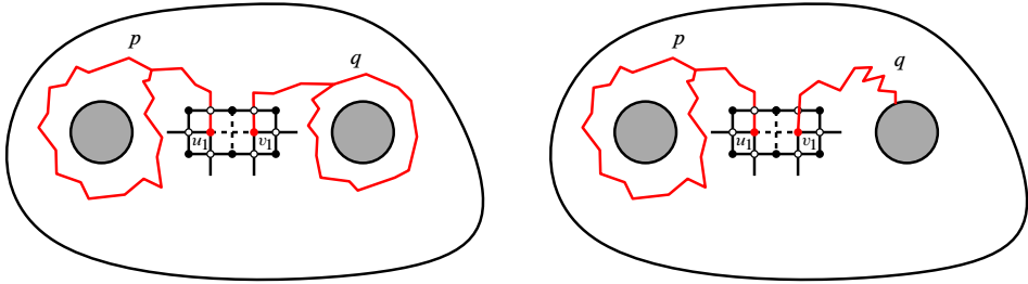
Figure 4. An illustration of the assumption in item (v). The paths \gamma_{u_1}, \gamma_{v_1} consist of p and q , which decompose the surface into a number of disconnected annuli: three in the first case and two in the second. The dotted edges are the ones removed from G to get G' .
