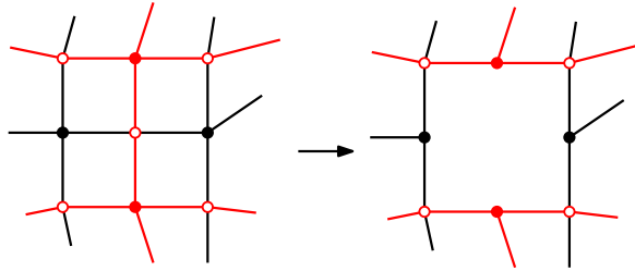
Figure 2. Removing a white vertex (puncture) to create the dimer graph G' .
