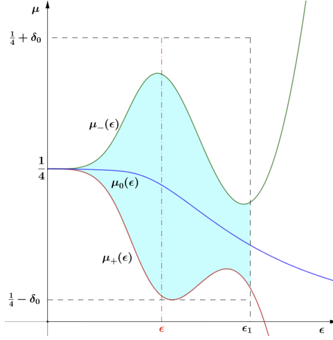
Figure 3. The degenerate instability region. We boxed with black dashed lines the validity box of Theorem 1. At any fixed \varepsilon , for (\mu, \varepsilon) in the colored cusp-shape region, one has the formation of the isola of instability in Figure 2.
