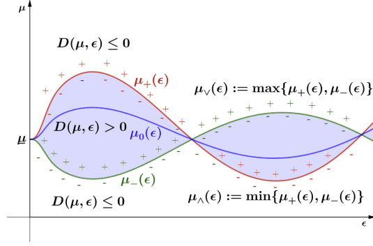
Figure 4. The instability region around the curve \mu_0(\epsilon) delimited by the curves \mu_v(\epsilon) and \mu_w(\epsilon) .
