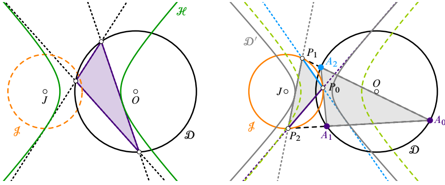
Figure 5. Left: a hyperbola, its director circle, and a secant director porism \{\mathcal{D}, \mathcal{H}\} . Right: the focal circle and the director circle form a secant Chapple porism \{\mathcal{D}, \mathcal{J}\} . The polars of the vertices A_0, A_1, A_2 with respect to \mathcal{J} are the sides of the poristic orbit P_0P_1P_2 , which envelops the hyperbola \mathcal{D}' , the polar dual of \mathcal{D} , with respect to \mathcal{J} .
