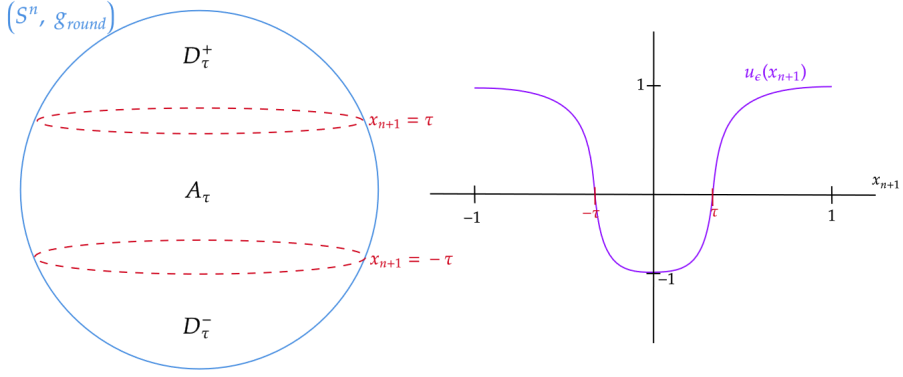
Figure 4. Example of matching Neumann data on the sphere
