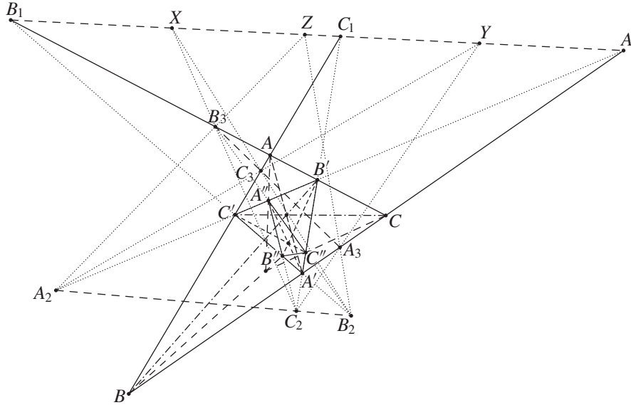
Fig. 2 Proof of Theorem 2.1
